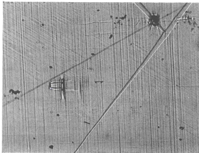
(a) (11\bar{2}0)
