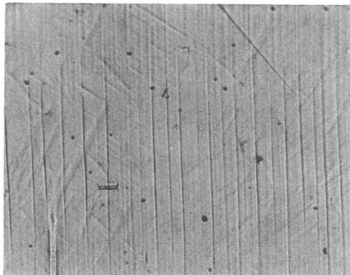
(b) (1010)
